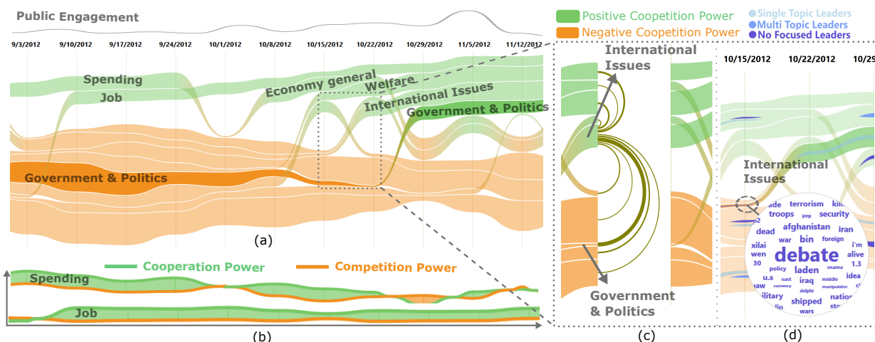
Fig. 1. (a) Topic coopetition dynamics during the 2012 U.S. presidential election with EvoRiver, showing most of the topics were transitioning from competition to cooperation during that time; (b) playfair-style chart of spending and job to unfold their coopetition power; (c) pairwise similarity between international issues and other topics with connected arcs; (d) word cloud of international issues .
